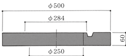
NHVO-25-60SS(A-B) (底板)
